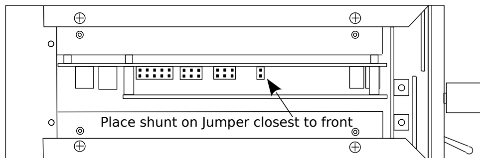
Figure 4-2. The Shunt Position to Enable Level 4 Access
