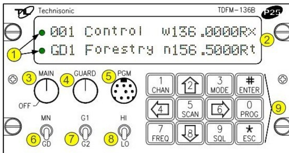
Figure 1-1. The TDFM-136B front panel showing control & display features.
