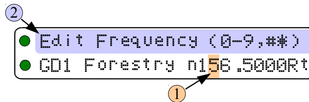
Figure 2-2. The user screen to edit the Guard frequency
